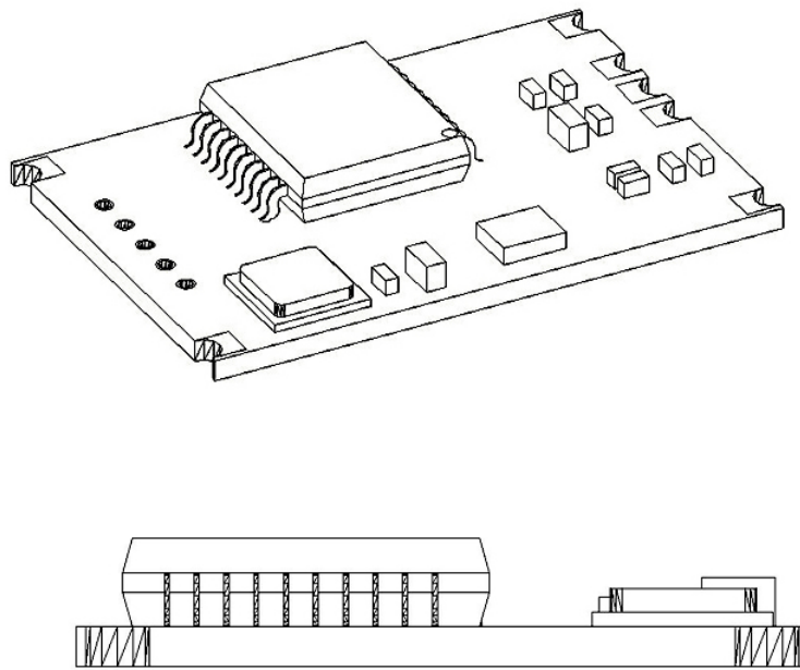
Figure 2: DSPC01 Dimensions
